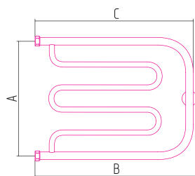
Аира 500x650 **0011-5065
